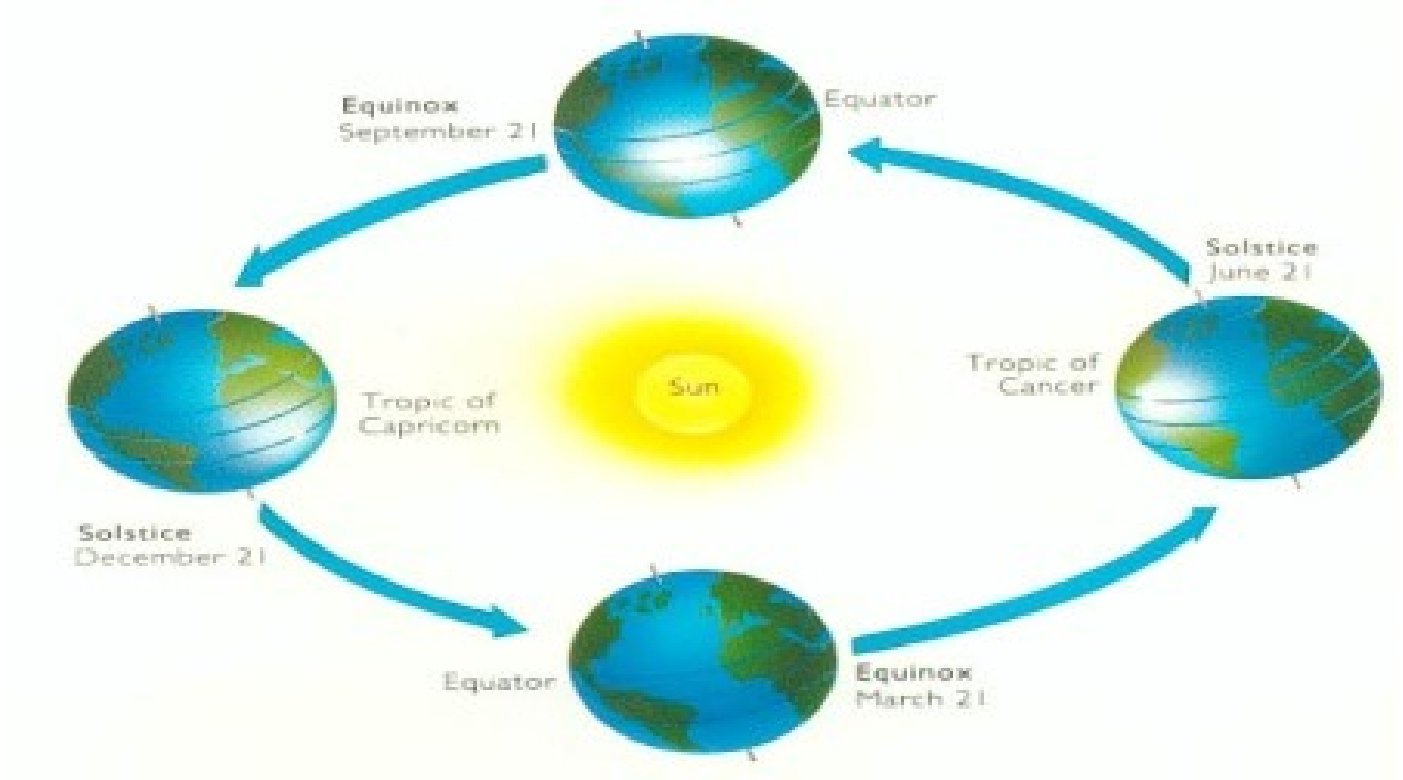
Earth orbital changes
